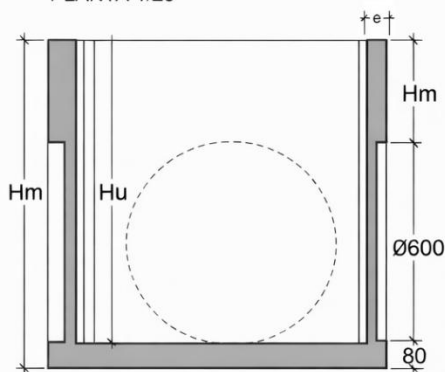
VISTA 1 1/20
